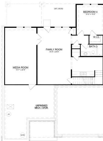
Finished Basement - Option 2 Bedroom, Bath, Family Room & Media
